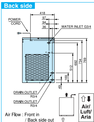
FM-600AHE w/B-300bin
