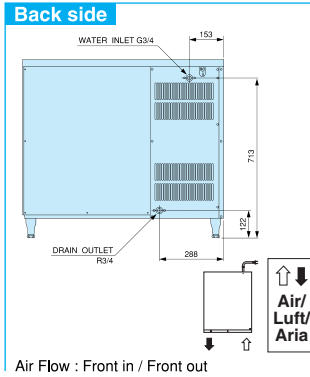
FM-600AHE w/B-300bin
