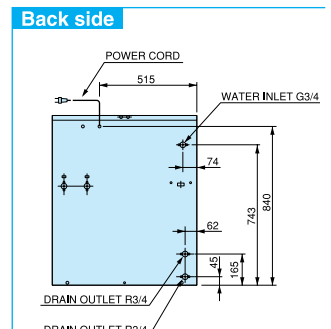
FM-1000ASFE3 w/B-900bin
