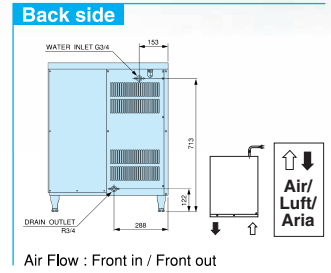
FM-251AFE w/B-300bin
